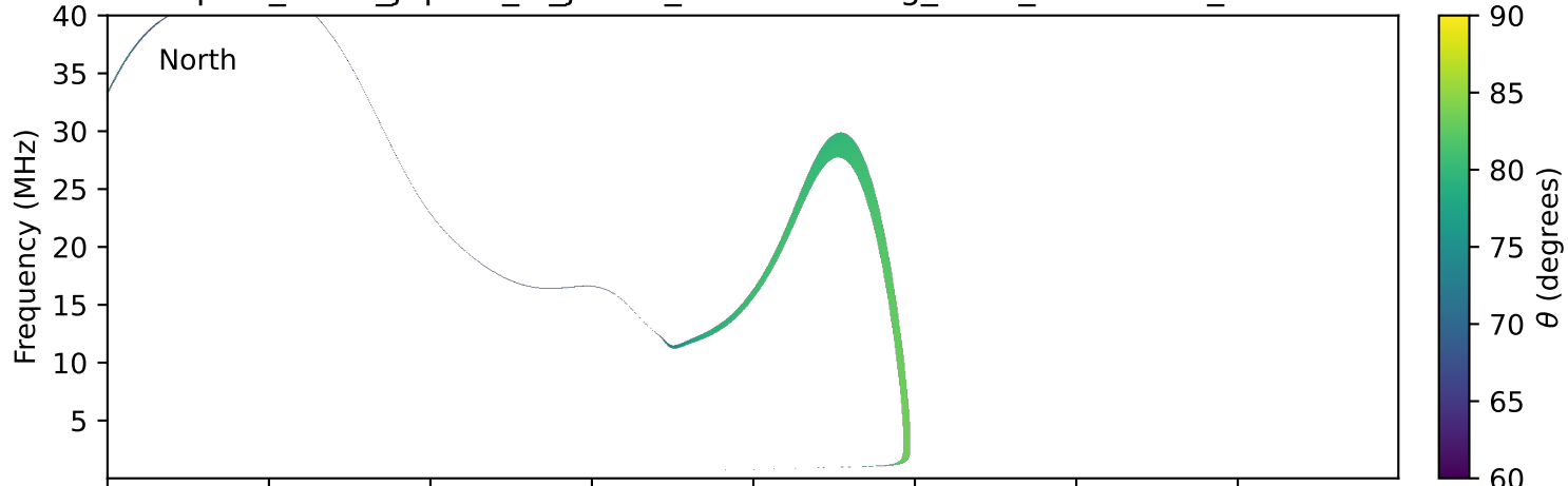
expres_earth_jupiter_io_jrm33_lossc-wid1deg_3kev_20190804_v11.cdf
