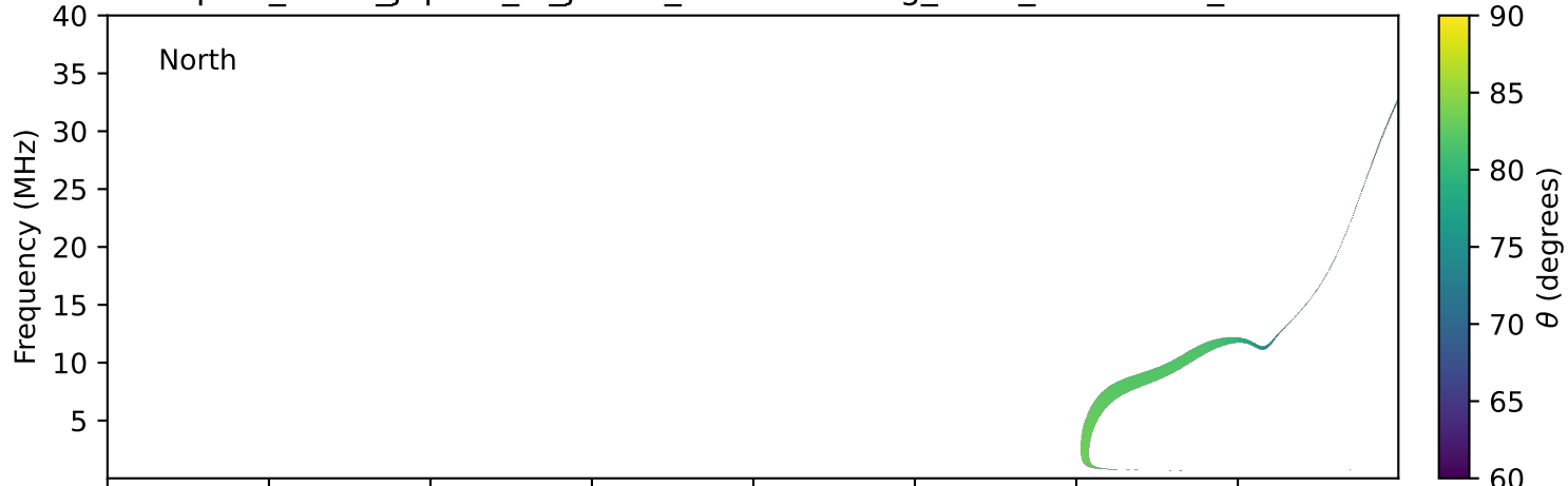
expres_earth_jupiter_io_jrm33_lossc-wid1deg_3kev_20190803_v11.cdf
