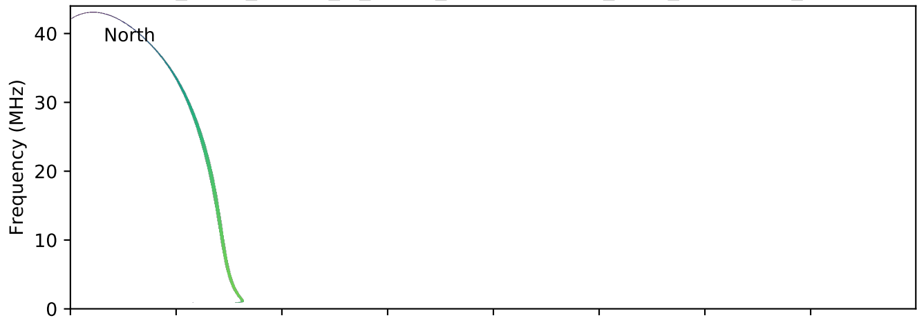
expres_earth_jupiter_io_jrm09_lossc-wid1deg_3kev_20190831_v01.cdf
