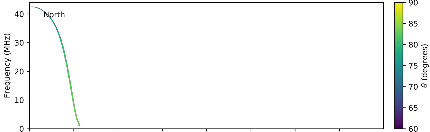
expres_earth_jupiter_io_jrm09_lossc-wid1deg_3kev_20190824_v01.cdf
