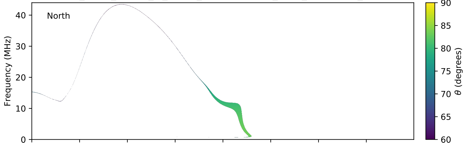
expres_earth_jupiter_io_jrm09_lossc-wid1deg_3kev_20190820_v01.cdf
