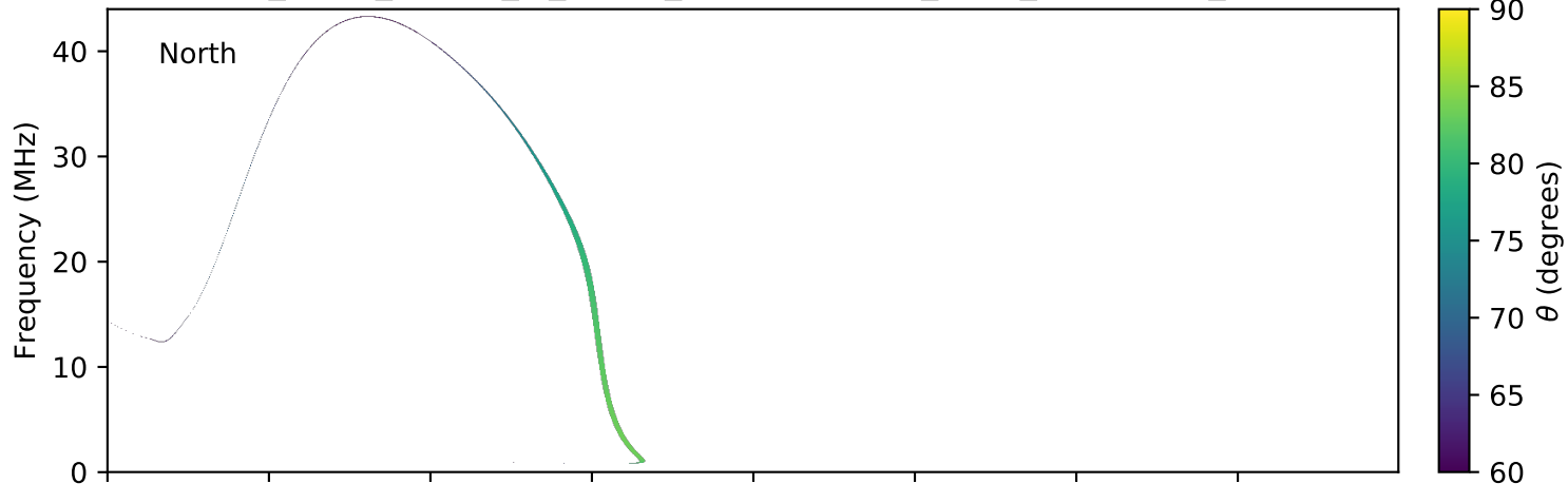
expres_earth_jupiter_io_jrm09_lossc-wid1deg_3kev_20190806_v01.cdf
