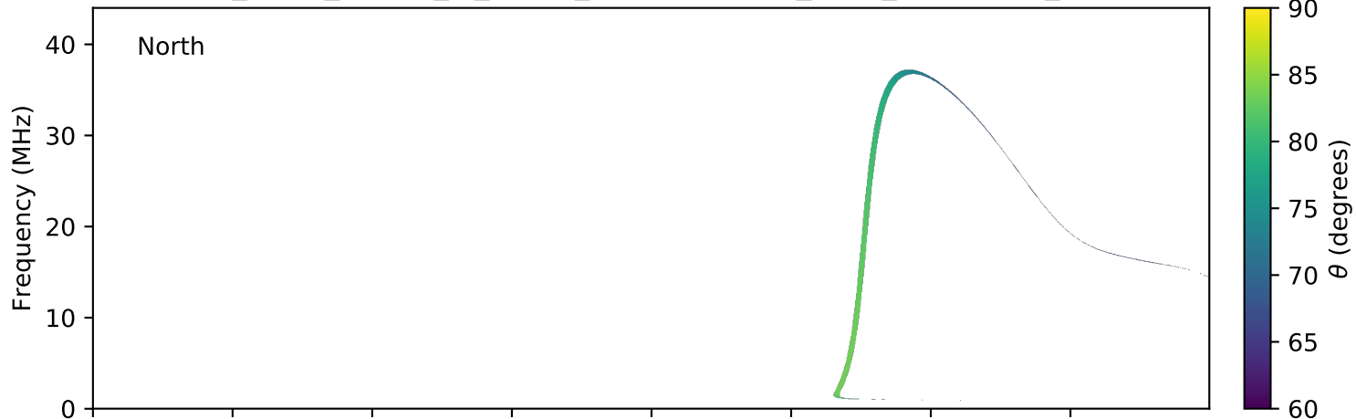
expres_earth_jupiter_io_jrm09_lossc-wid1deg_3kev_20190805_v01.cdf
