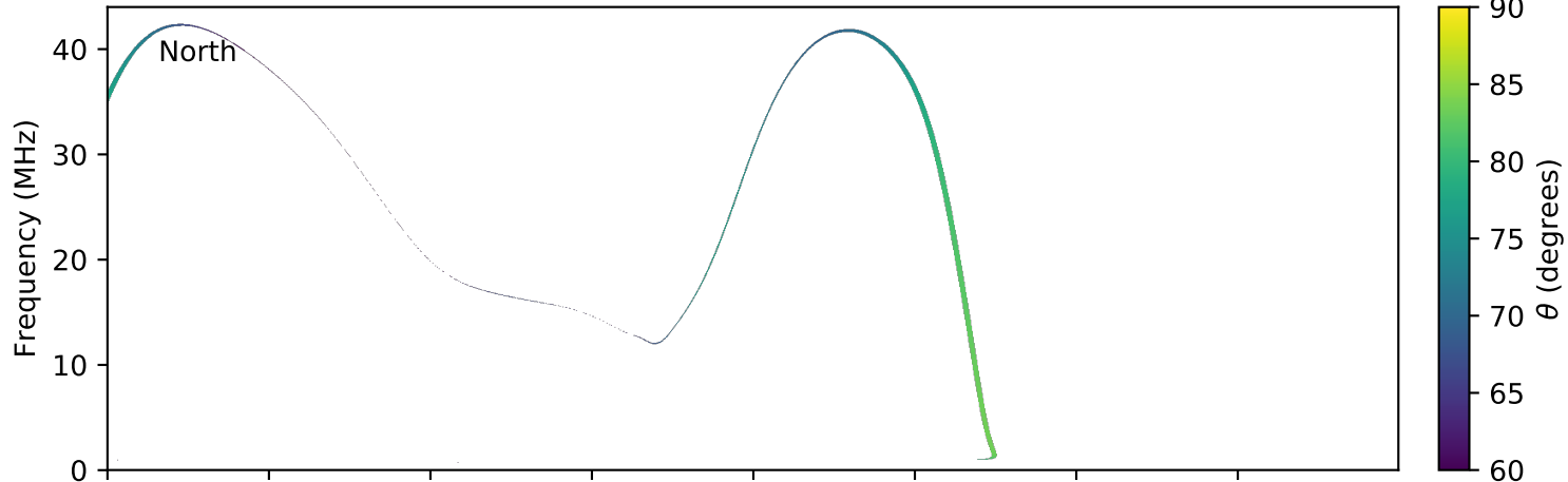
expres_earth_jupiter_io_jrm09_lossc-wid1deg_3kev_20190804_v01.cdf
