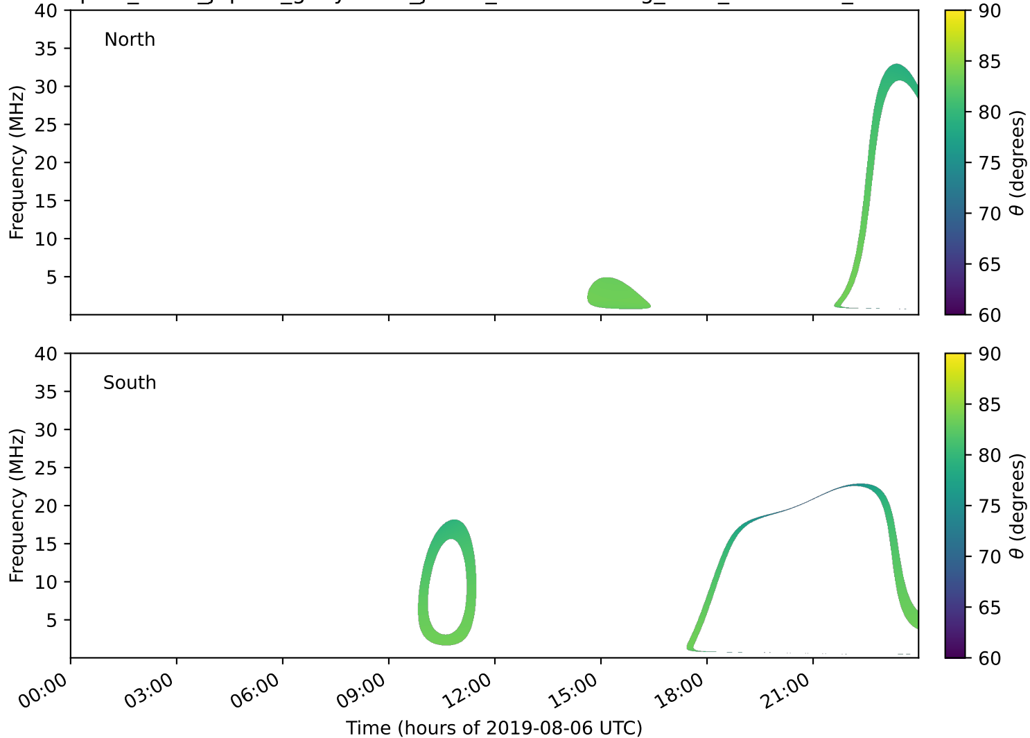
expres_earth_jupiter_ganymede_jrm33_lossc-wid1deg_3kev_20190806_v11.cdf
