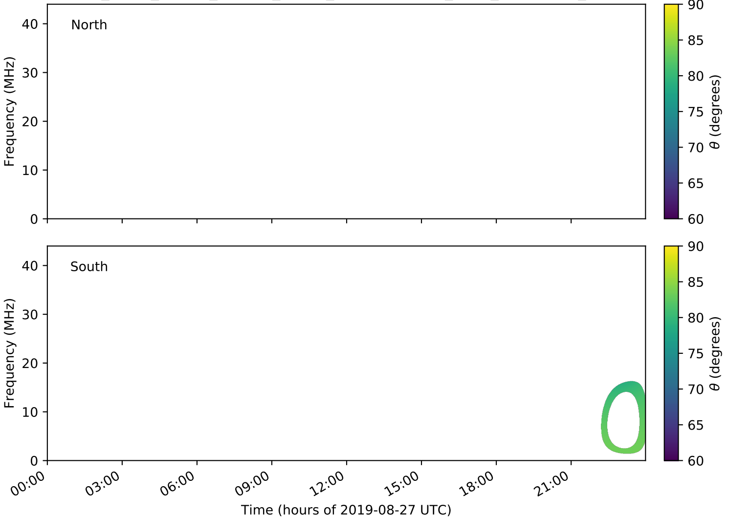
expres_earth_jupiter_europa_jrm09_lossc-wid1deg_3kev_20190827_v01.cdf
