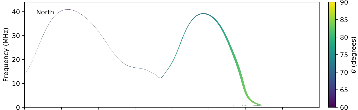
expres_earth_jupiter_europa_jrm09_lossc-wid1deg_3kev_20190811_v01.cdf
