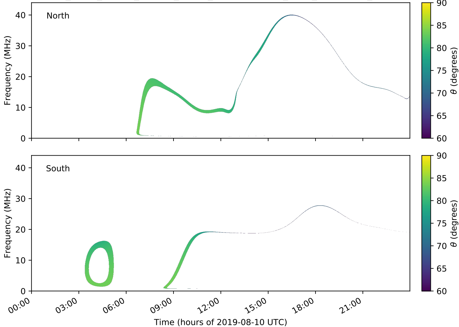
expres_earth_jupiter_europa_jrm09_lossc-wid1deg_3kev_20190810_v01.cdf
