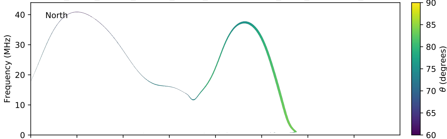
expres_earth_jupiter_europa_jrm09_lossc-wid1deg_3kev_20190804_v01.cdf
