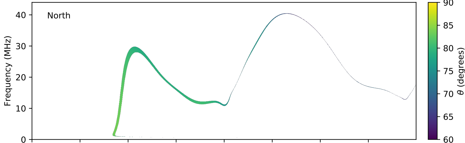
expres_earth_jupiter_europa_jrm09_lossc-wid1deg_3kev_20190803_v01.cdf
