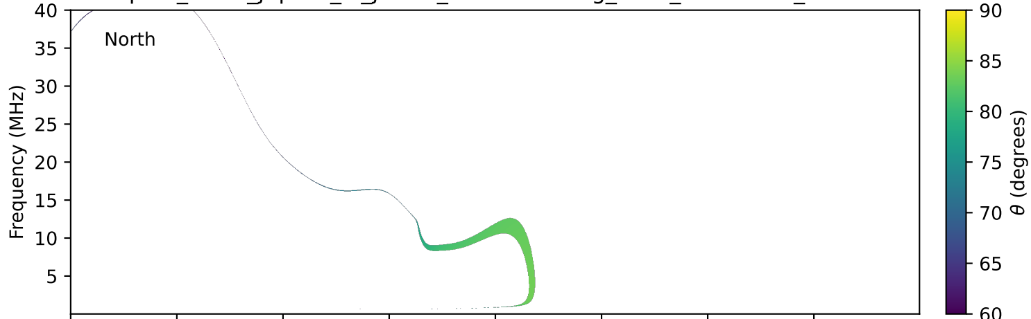
expres_earth_jupiter_io_jrm33_lossc-wid1deg_3kev_20190728_v11.cdf
