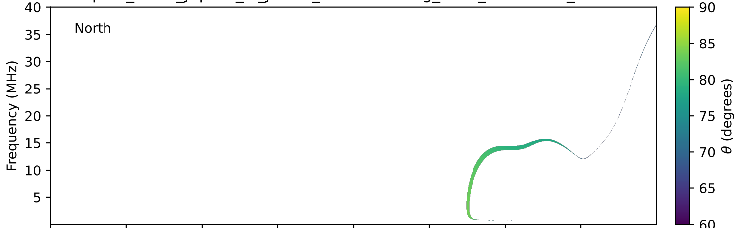
expres_earth_jupiter_io_jrm33_lossc-wid1deg_3kev_20190727_v11.cdf
