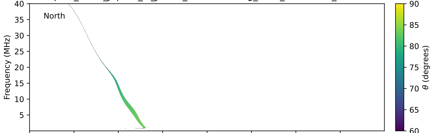
expres_earth_jupiter_io_jrm33_lossc-wid1deg_3kev_20190714_v11.cdf
