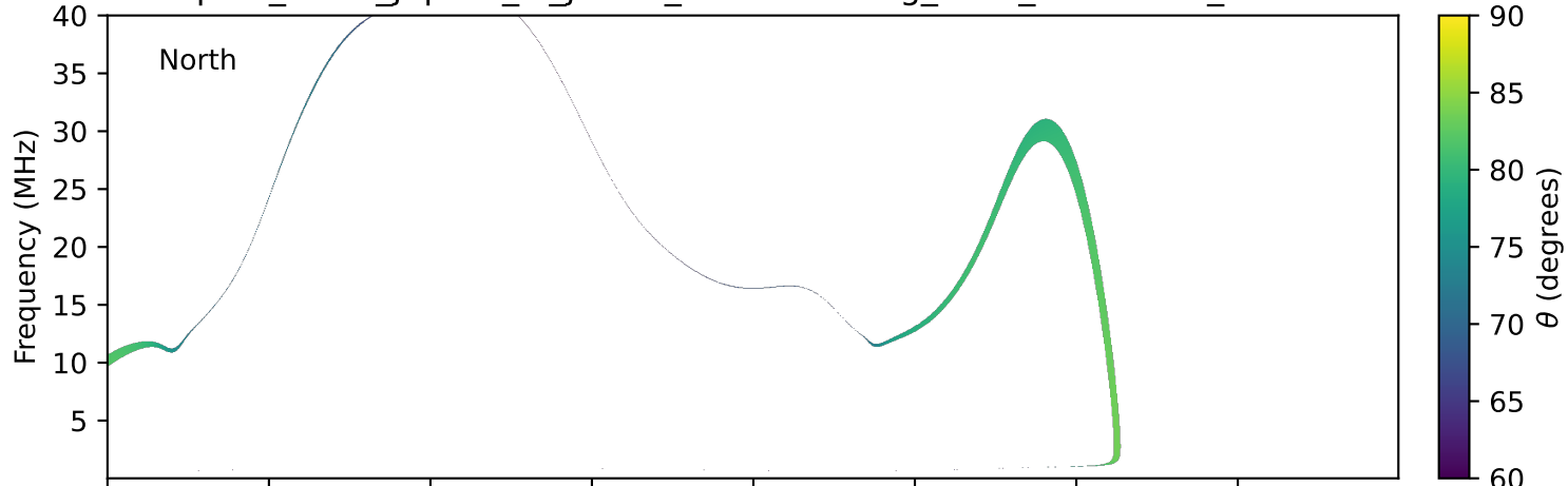
expres_earth_jupiter_io_jrm33_lossc-wid1deg_3kev_20190703_v11.cdf
