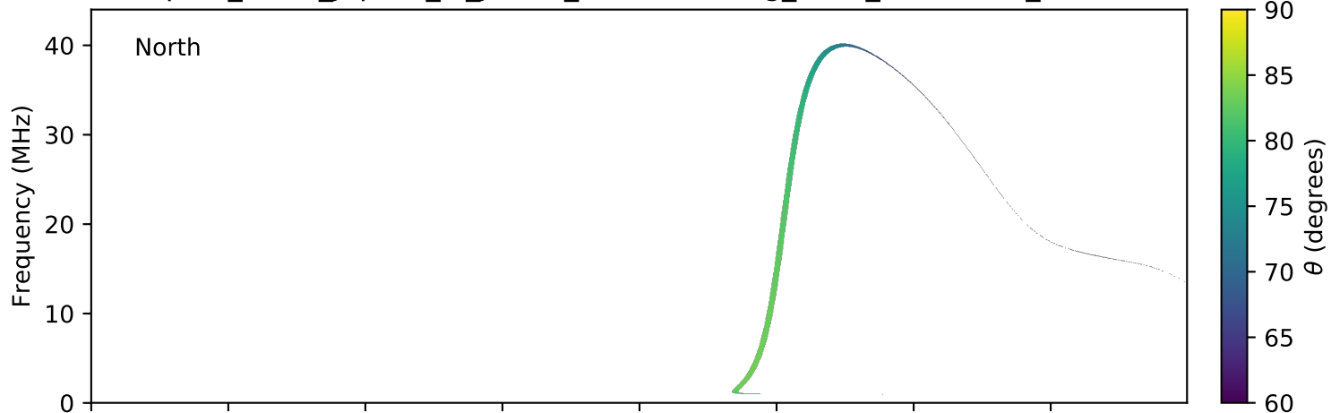
expres_earth_jupiter_io_jrm09_lossc-wid1deg_3kev_20190729_v01.cdf
