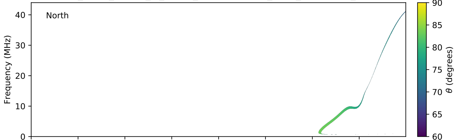
expres_earth_jupiter_io_jrm09_lossc-wid1deg_3kev_20190727_v01.cdf
