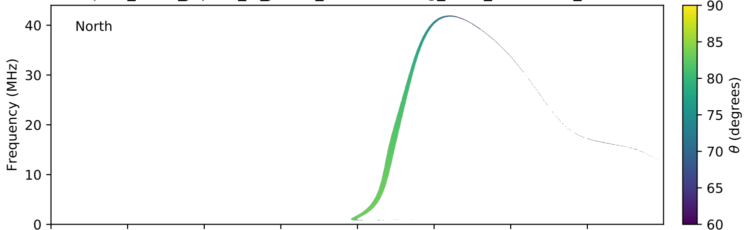
expres_earth_jupiter_io_jrm09_lossc-wid1deg_3kev_20190722_v01.cdf
