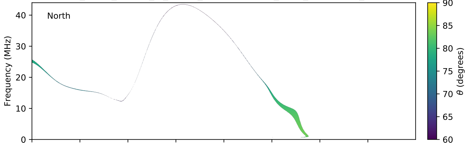
expres_earth_jupiter_io_jrm09_lossc-wid1deg_3kev_20190719_v01.cdf
