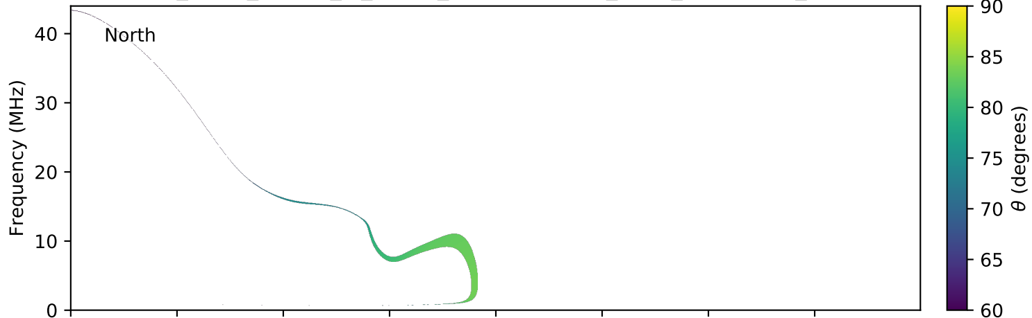
expres_earth_jupiter_io_jrm09_lossc-wid1deg_3kev_20190714_v01.cdf
