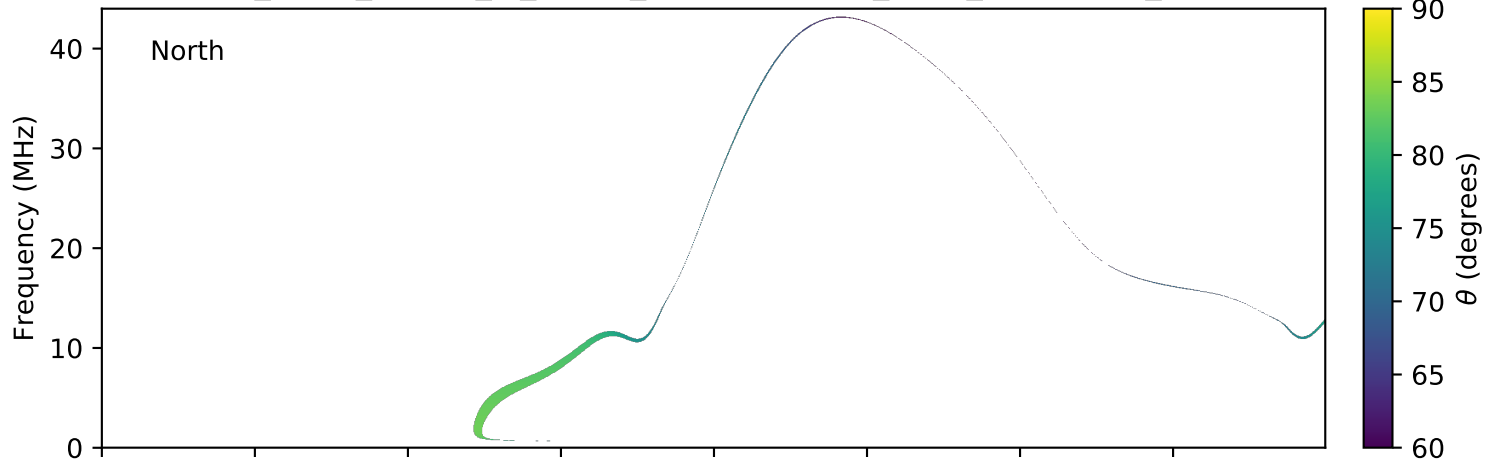
expres_earth_jupiter_io_jrm09_lossc-wid1deg_3kev_20190708_v01.cdf
