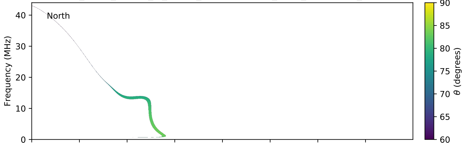
expres_earth_jupiter_io_jrm09_lossc-wid1deg_3kev_20190707_v01.cdf
