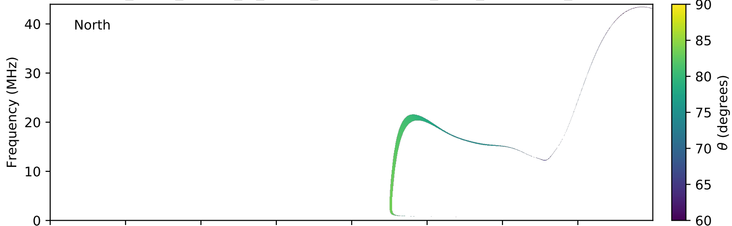
expres_earth_jupiter_io_jrm09_lossc-wid1deg_3kev_20190706_v01.cdf
