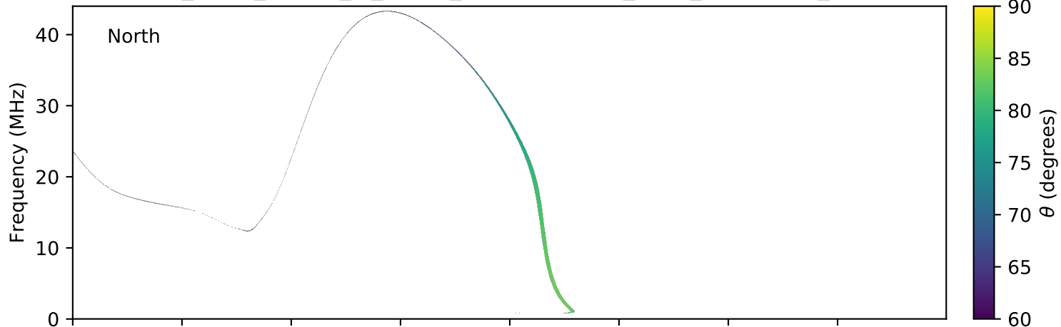
expres_earth_jupiter_io_jrm09_lossc-wid1deg_3kev_20190705_v01.cdf
