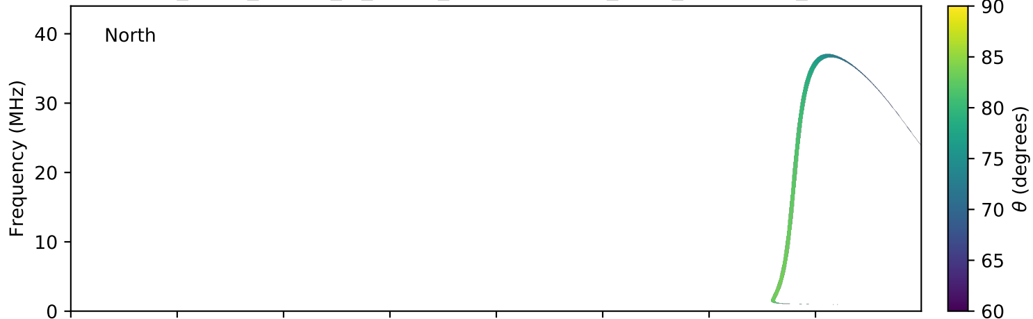
expres_earth_jupiter_io_jrm09_lossc-wid1deg_3kev_20190704_v01.cdf
