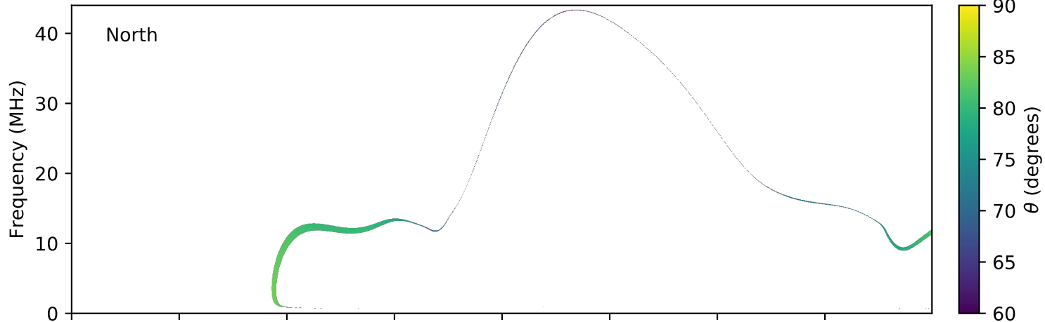
expres_earth_jupiter_io_jrm09_lossc-wid1deg_3kev_20190701_v01.cdf
