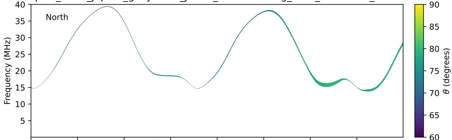
expres_earth_jupiter_ganymede_jrm33_lossc-wid1deg_3kev_20190718_v11.cdf
