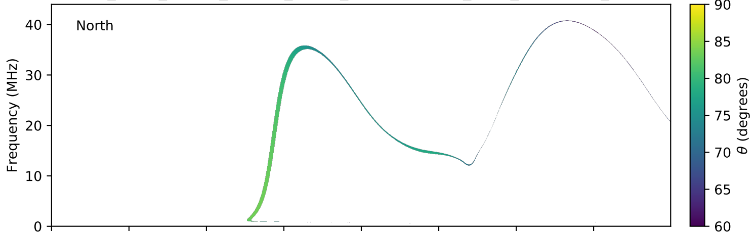
expres_earth_jupiter_europa_jrm09_lossc-wid1deg_3kev_20190702_v01.cdf
