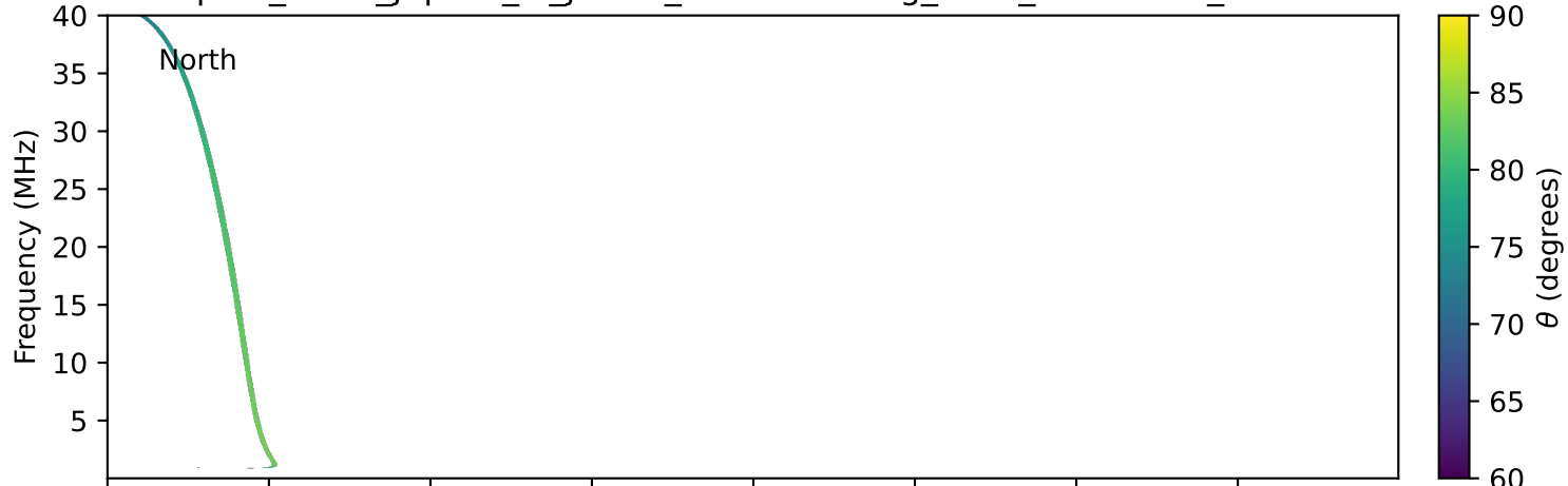
expres_earth_jupiter_io_jrm33_lossc-wid1deg_3kev_20190623_v11.cdf
