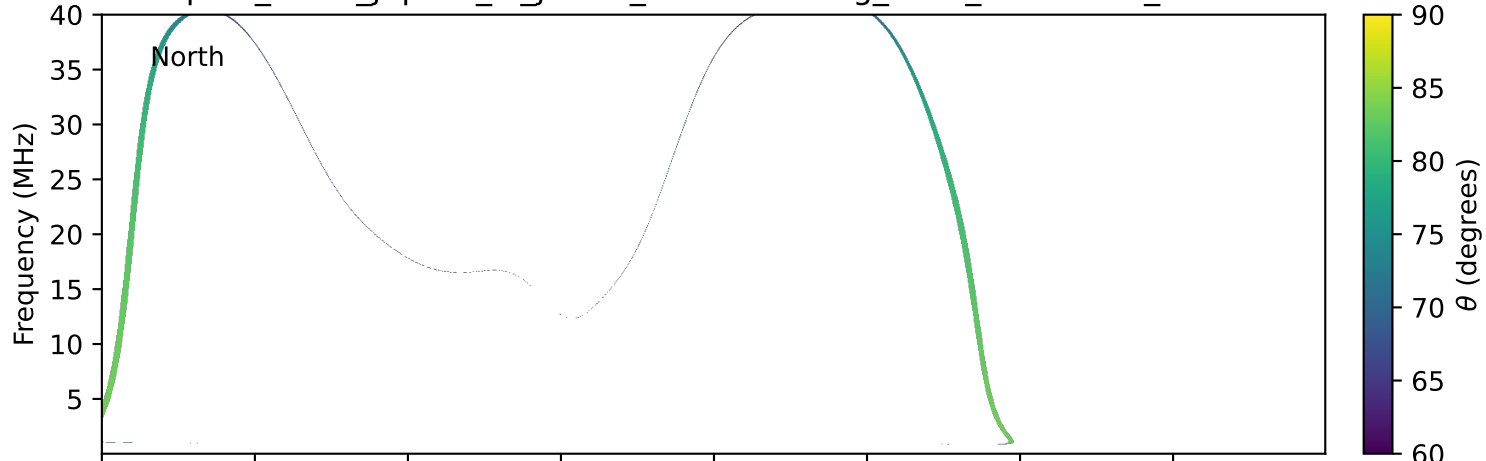
expres_earth_jupiter_io_jrm33_lossc-wid1deg_3kev_20190610_v11.cdf
