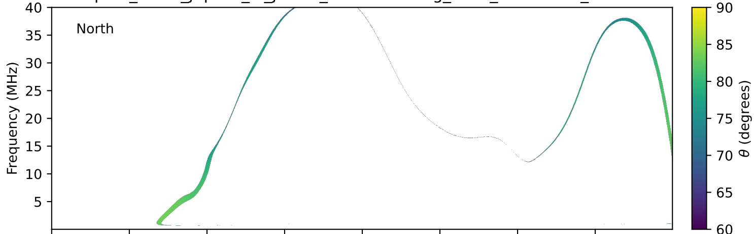
expres_earth_jupiter_io_jrm33_lossc-wid1deg_3kev_20190608_v11.cdf
