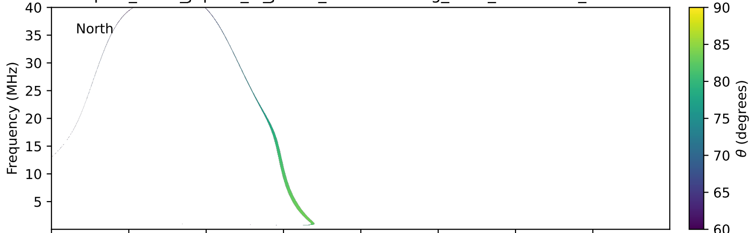
expres_earth_jupiter_io_jrm33_lossc-wid1deg_3kev_20190605_v11.cdf
