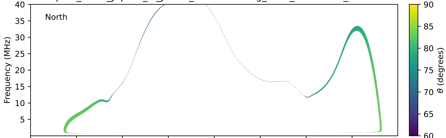
expres_earth_jupiter_io_jrm33_lossc-wid1deg_3kev_20190601_v11.cdf
