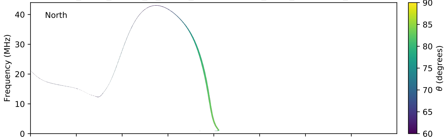
expres_earth_jupiter_io_jrm09_lossc-wid1deg_3kev_20190628_v01.cdf
