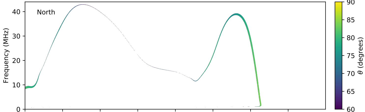
expres_earth_jupiter_io_jrm09_lossc-wid1deg_3kev_20190626_v01.cdf
