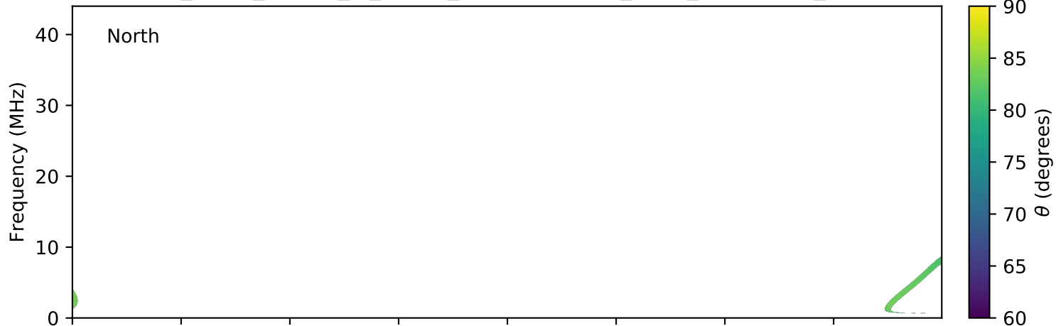
expres_earth_jupiter_io_jrm09_lossc-wid1deg_3kev_20190625_v01.cdf
