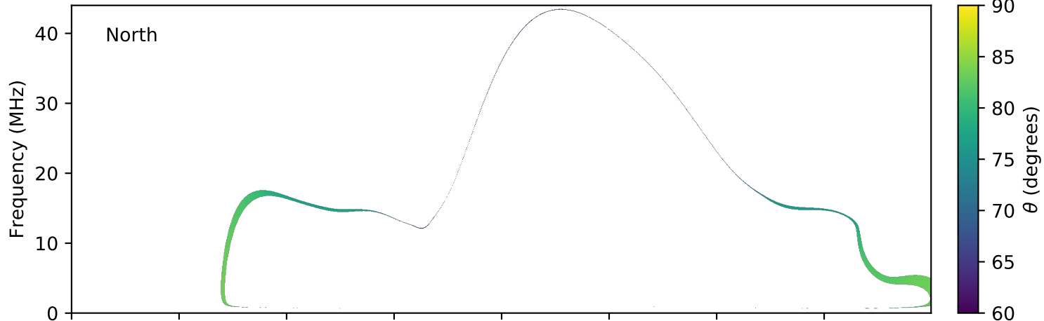
expres_earth_jupiter_io_jrm09_lossc-wid1deg_3kev_20190624_v01.cdf
