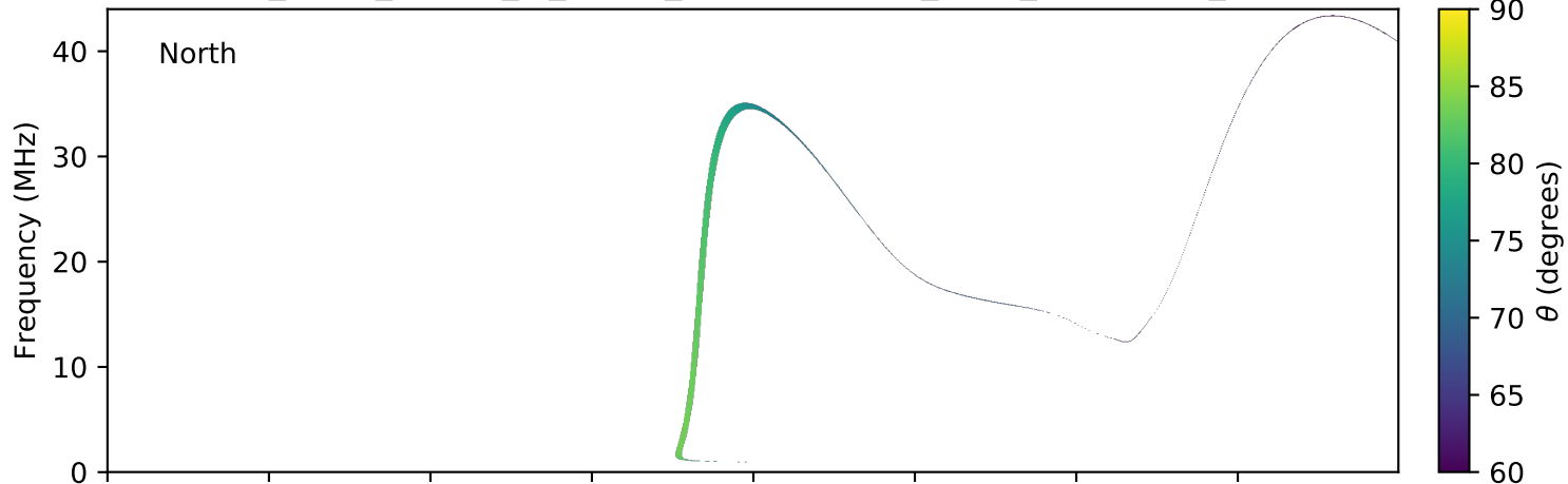
expres_earth_jupiter_io_jrm09_lossc-wid1deg_3kev_20190622_v01.cdf
