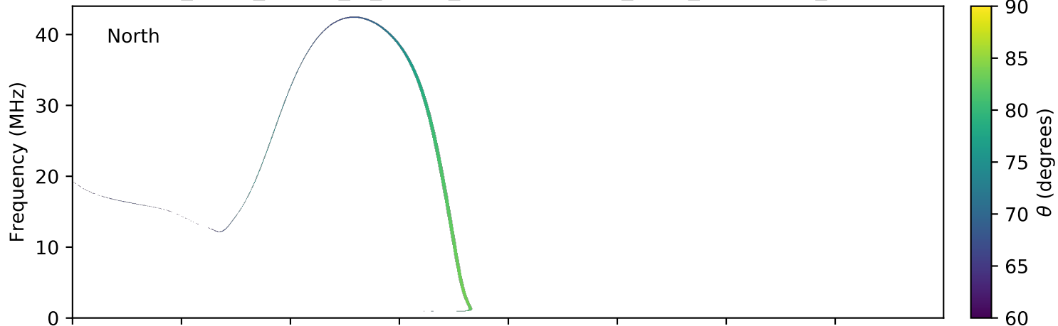
expres_earth_jupiter_io_jrm09_lossc-wid1deg_3kev_20190621_v01.cdf
