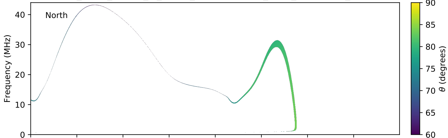
expres_earth_jupiter_io_jrm09_lossc-wid1deg_3kev_20190619_v01.cdf
