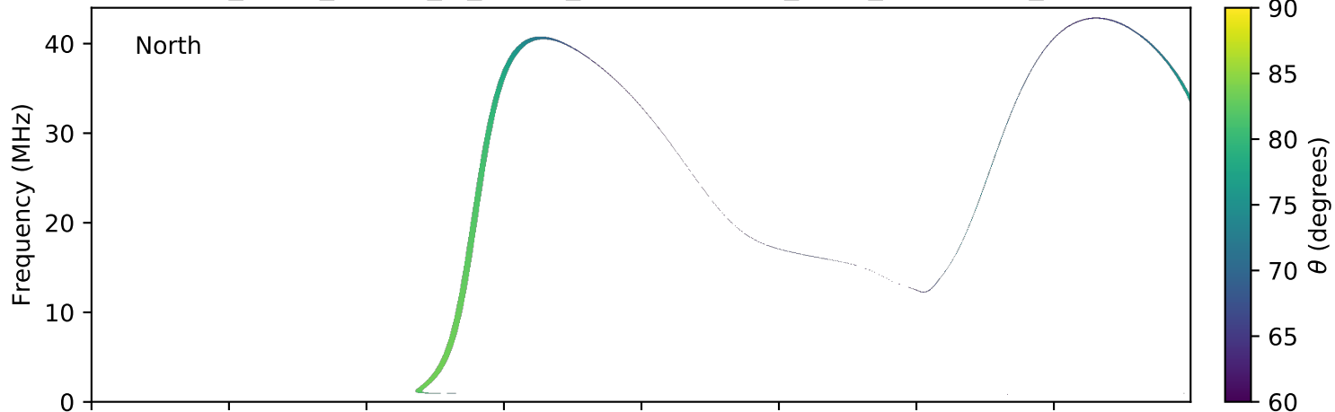
expres_earth_jupiter_io_jrm09_lossc-wid1deg_3kev_20190608_v01.cdf
