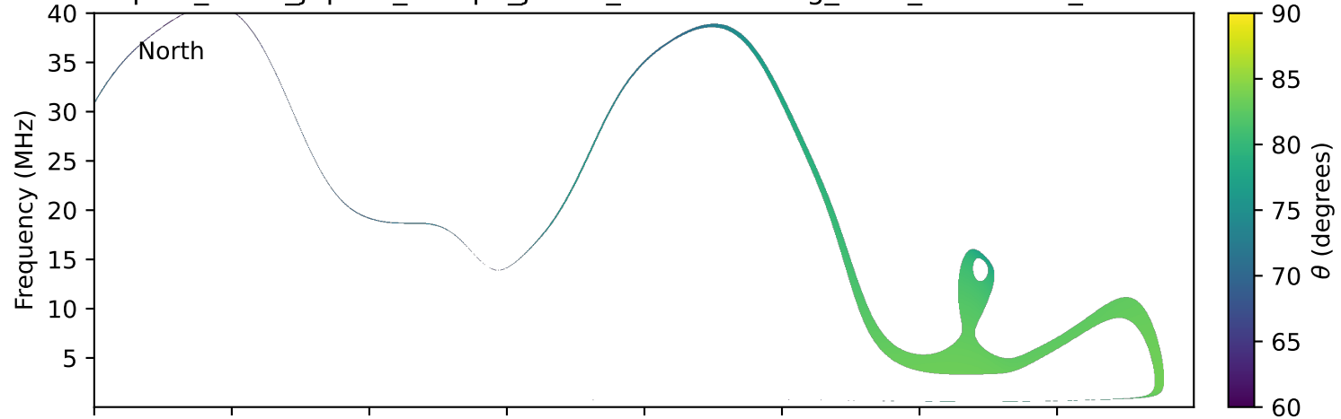
expres_earth_jupiter_europa_jrm33_lossc-wid1deg_3kev_20190615_v11.cdf
