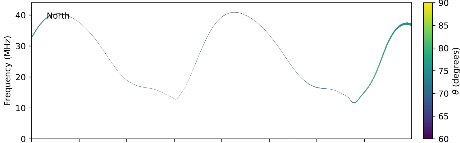
expres_earth_jupiter_europa_jrm09_lossc-wid1deg_3kev_20190622_v01.cdf
