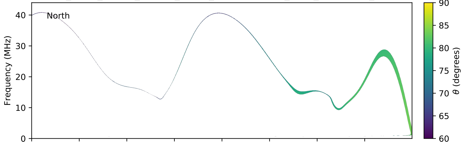
expres_earth_jupiter_europa_jrm09_lossc-wid1deg_3kev_20190608_v01.cdf
