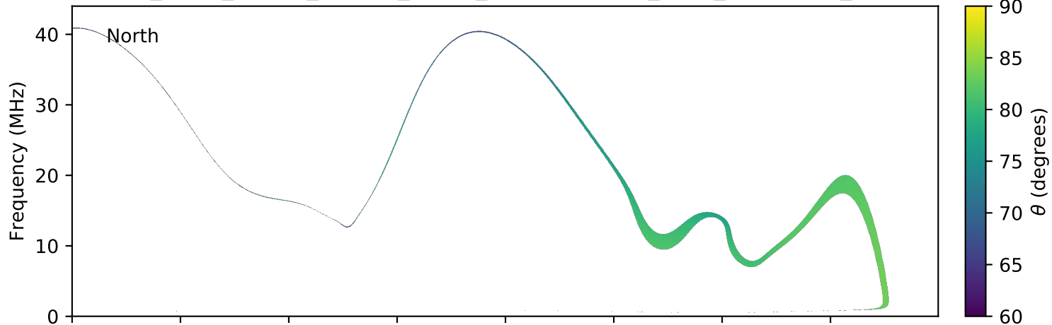
expres_earth_jupiter_europa_jrm09_lossc-wid1deg_3kev_20190601_v01.cdf
