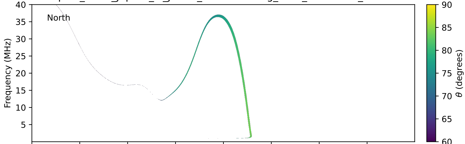
expres_earth_jupiter_io_jrm33_lossc-wid1deg_3kev_20190520_v11.cdf
