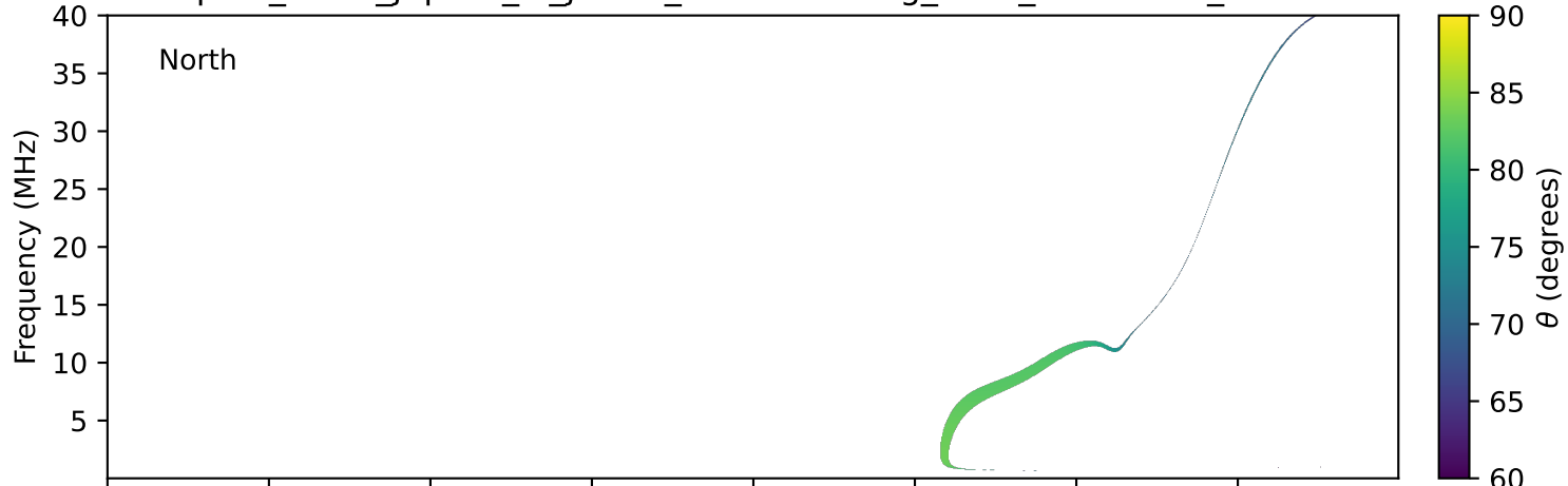
expres_earth_jupiter_io_jrm33_lossc-wid1deg_3kev_20190512_v11.cdf
